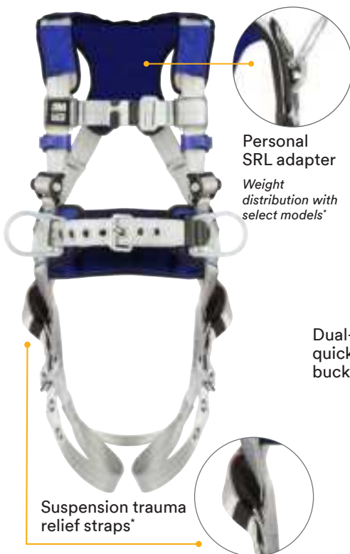
3M™ DBI-SALA® ExoFit™ X100 Harness
