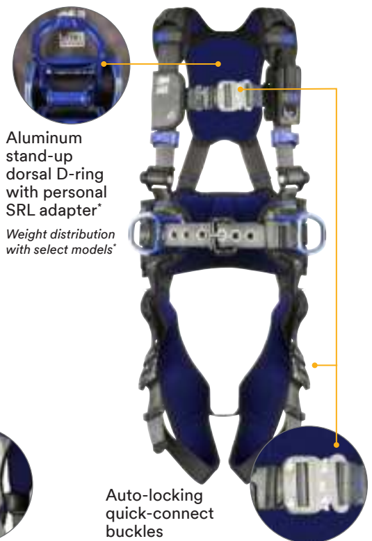
3M™ DBI-SALA® ExoFit™ X300 Harness
